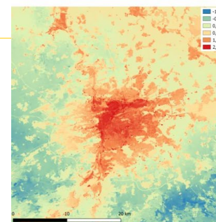
ERA5 2011-2020 Reference
